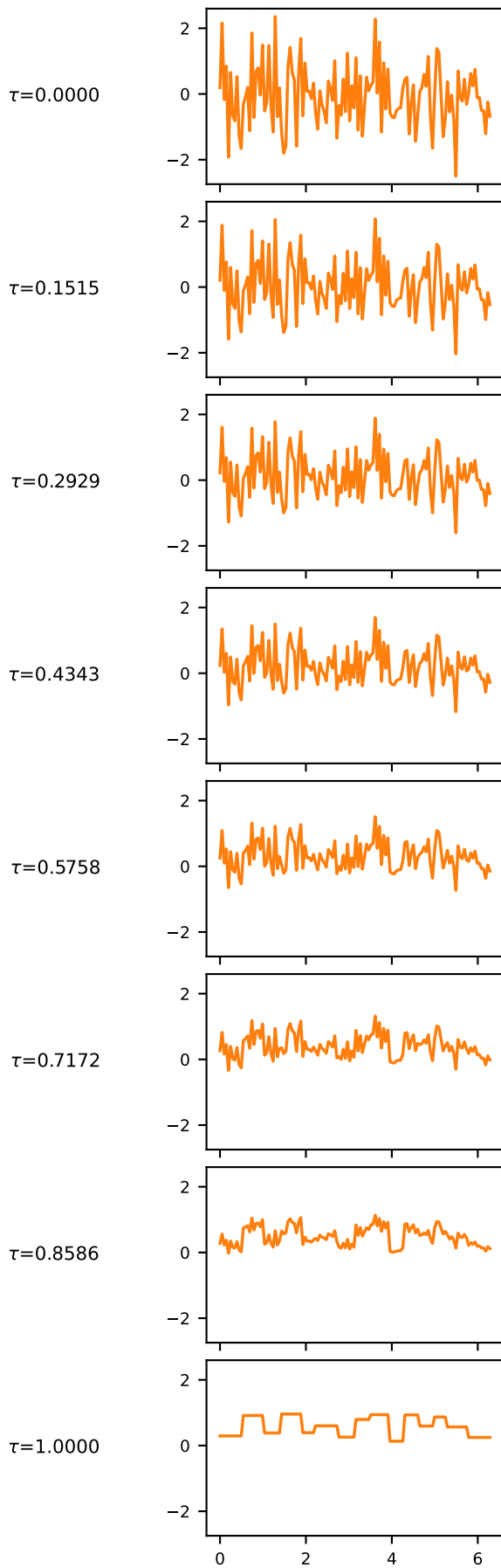
Flow matching
